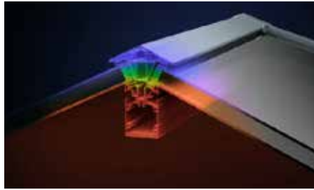
28mm glazing units with 1.0 Wm 2 K U-Value
