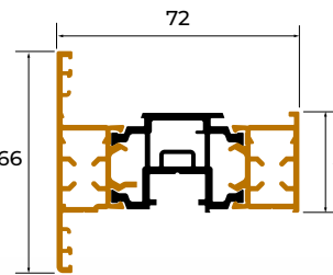
SP301 CONTEMPORARY SASH
