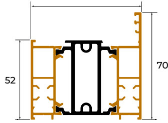
SP104 LARGE OUTER FRAME
