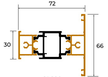
SP200 TRANSOM/MULLION
