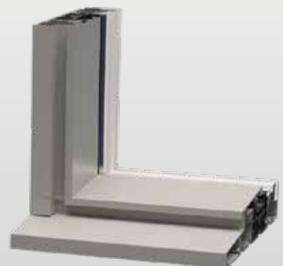
Standard outer frame with clip-on cill nose
