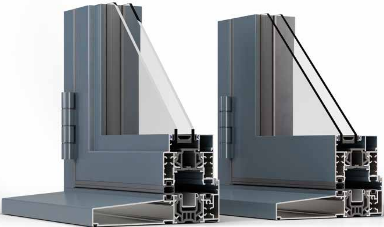
Stepped sash
