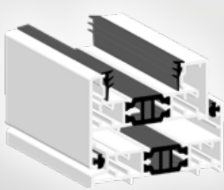
Contemporary sash, Flush frame
