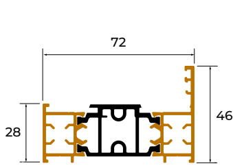
SP100 SMALL OUTER FRAME
