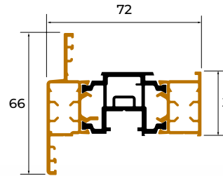
SP301 STEPPED SASH
