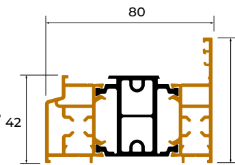
SP103 INTERMEDIATE FLUSH OUTER FRAME
