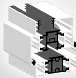
Stepped sash, Standard frame
