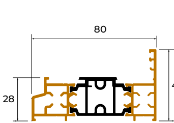
SP101 SMALL FLUSH OUTER FRAME
