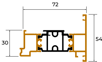
SP250 MEETING STILE
